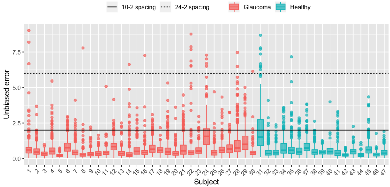
Supplementary Figure. Box-plots of the unbiased error for each subject. The boxes include the interquartile range, the whiskers extend to the 95% quantiles and the horizontal midline represents the median. The two horizontal black lines represent the spacing between locations of a 10-2 grid and of a 24-2 grid as a reference.
