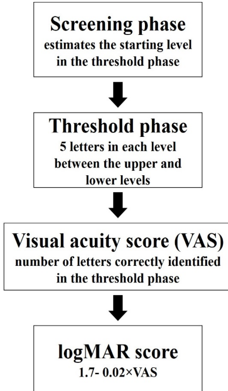
Figure S4. The E-ETDRS method 17 . The method has a screening phase and a threshold phase. The screening phase provides a coarse estimate of the observer's VA and the size range of optotype sizes to be tested in the threshold phase. The threshold phase is used to obtain a more precise estimate of VA.
