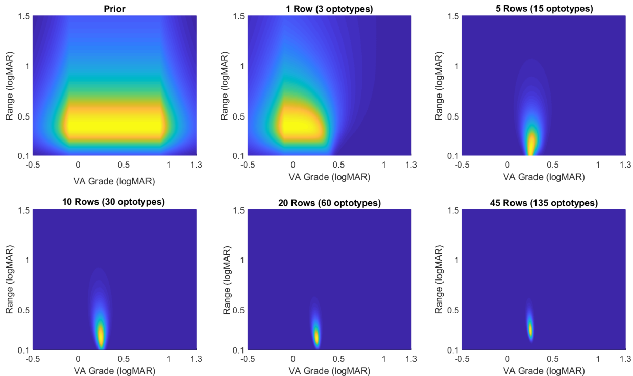
Figure S2. Illustration of the convergence of the joint probability distribution in one simulated qVA run. Each panel shows a heatmap of the joint probability distribution of acuity and range after the number of rows (and letters) shown in the caption.
