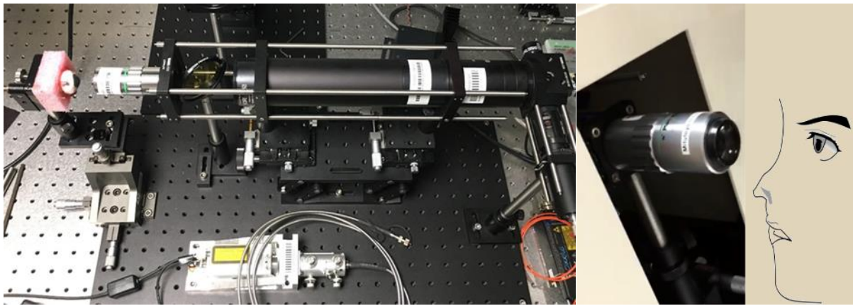
Fig. S1: Photograph and imaging concept of the developed prototype
