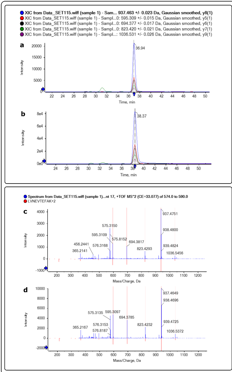
Supplementary Figure S2. The extracted ion chromatograms (XIC) (a, b) and associated mass spectra (c, d) for albumin (ALB). From the paired graphs, the top ones present specific capillary sample's results (a, c) and the lower graphs show the Schirmer strip samples results for the same subject (b, d). ALB has a higher expression level in the Schirmer strip sample.
