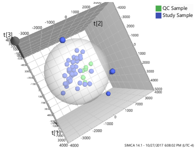
Fig S1. PCA plot of the post-surgical samples and the QC samples. The pre-surgical samples were not included in the QC pools due to limited volume.
