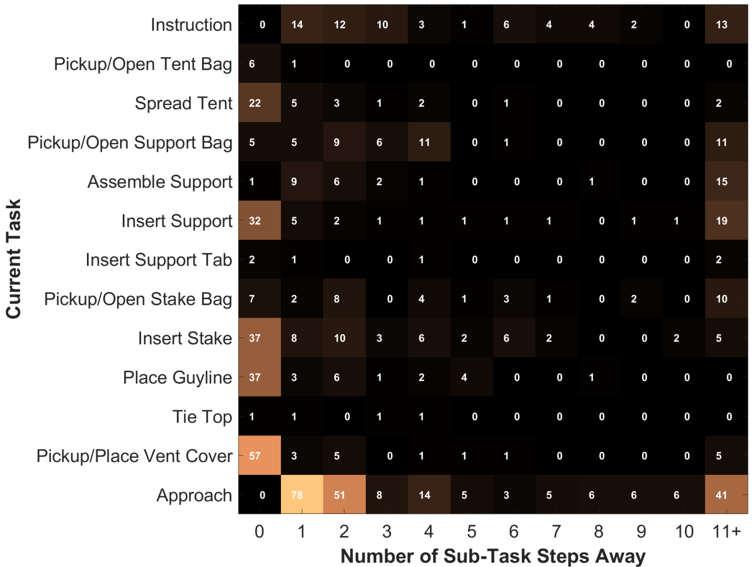
Figure A3. Frequency of LAFs as a function of task-steps. Rows indicate sub-tasks and each column entry indicates the number of LAFs occurring in that subtask and the number of sub-task steps ahead the LAF was directed. A sub-task step of zero means the LAF was directed within the ongoing sub-task. LAFs are primarily directed to other objects within 10 task steps but can go well beyond (~50 in the extreme)
