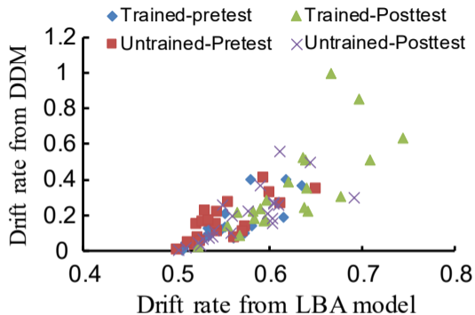
Figure S4. Drift rate estimated by the classical drift diffusion model. (A) Averaged drift rate across participants showed a specific enhancement in the trained direction, which is similar with the results from the LBA model. (B) Positive correlation ( r > 0.762 for all four conditions, p < 0.001 for all four experimental conditions) between the drift rate estimated by LBA model and DDM model.
