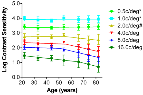
Supplementary Figure 4: Comparison to previous contrast sensitivity data
