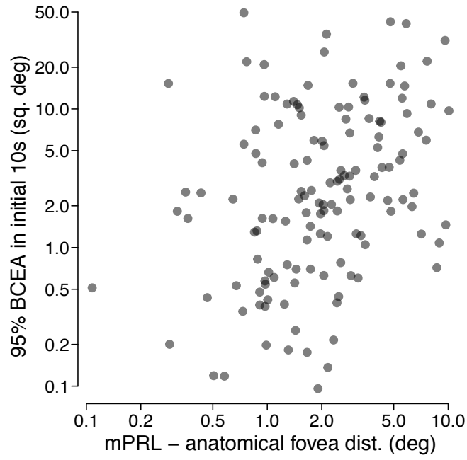
Supplementary Figure S1: Relationship between the distance between the mPRL and the anatomical fovea and the fixation stability in the initial 10s period used to determine the mPRL, as measured by 95% bivariate contour ellipse area (BCEA).
