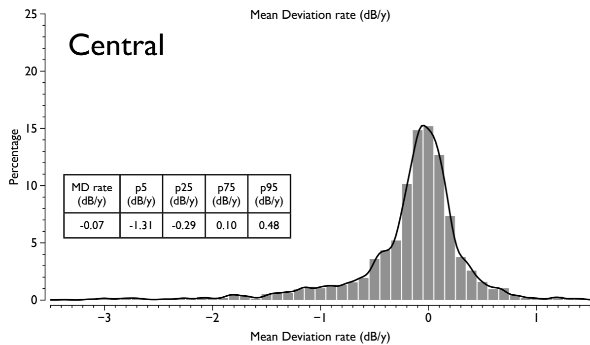
Supplementary Figure S1: Distribution of sectoral Mean Deviation (MD) rates in all 2,324 patients in the study. Also shown is the median MD rate and the 5 th , 25 th , 75 th and 95 th percentiles of the distributions. Curved line represents a spline fit of the histogram.
